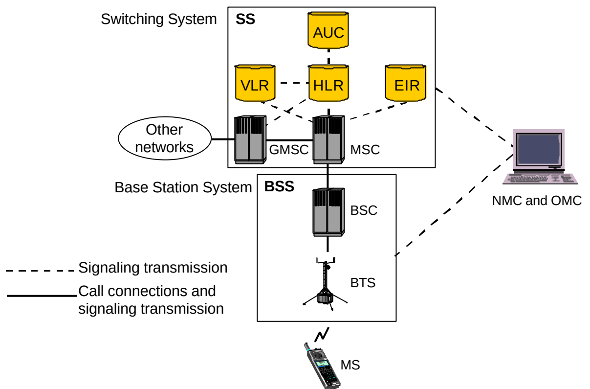
Figure 1-5 System model
